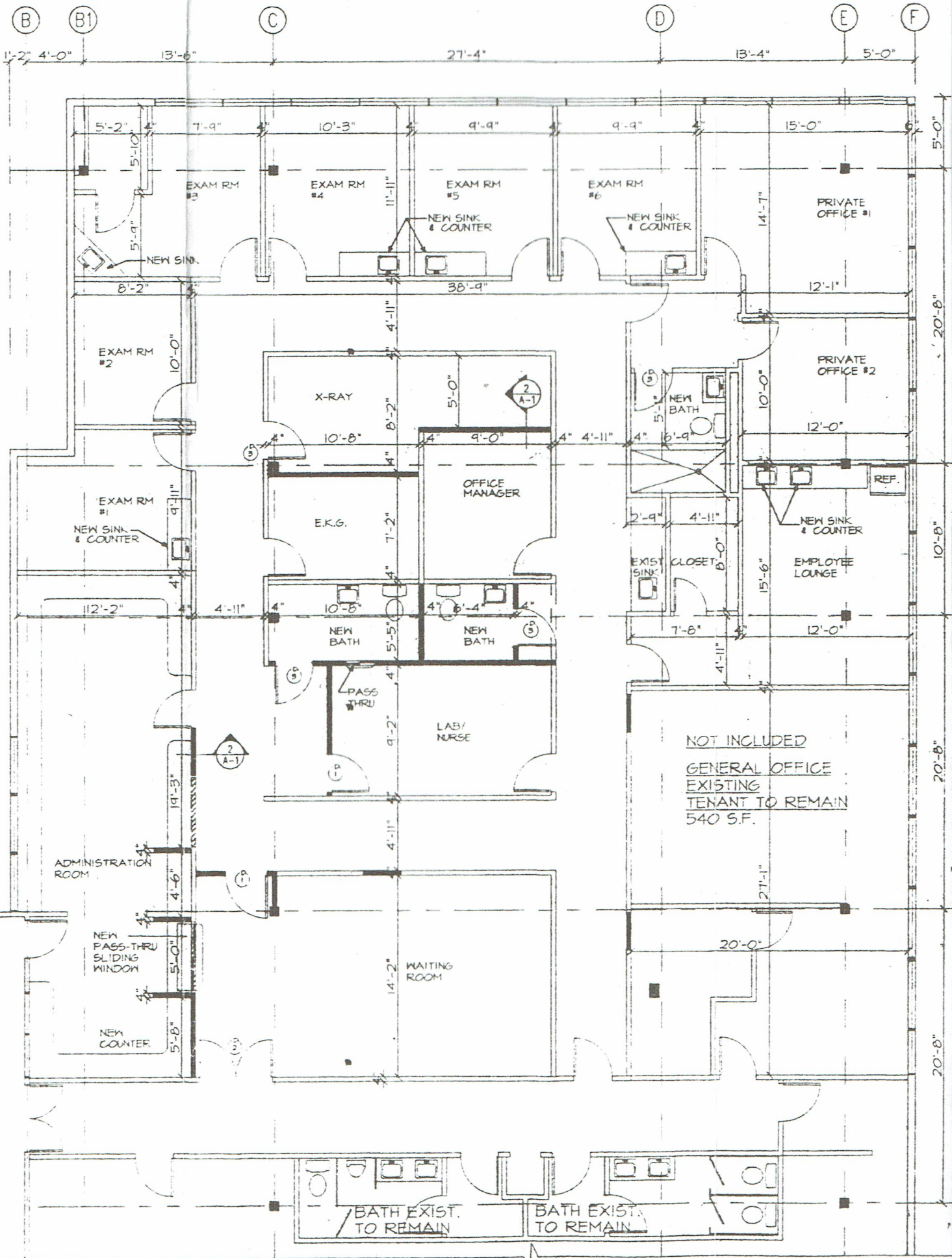
FLOOR PLAN 1/4" = 1'-0"
